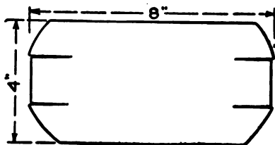
FIG. 211. — Pattern of Canopy-Top.
